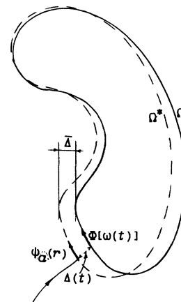
FIG. 1. The schematic view of the attractor \Omega^* and the considered manifold \Omega .
