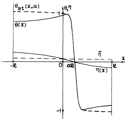
FIG. 3. The fragment of the dissipative structure placed in the interval [-\mathcal{L}, \mathcal{L}] .
